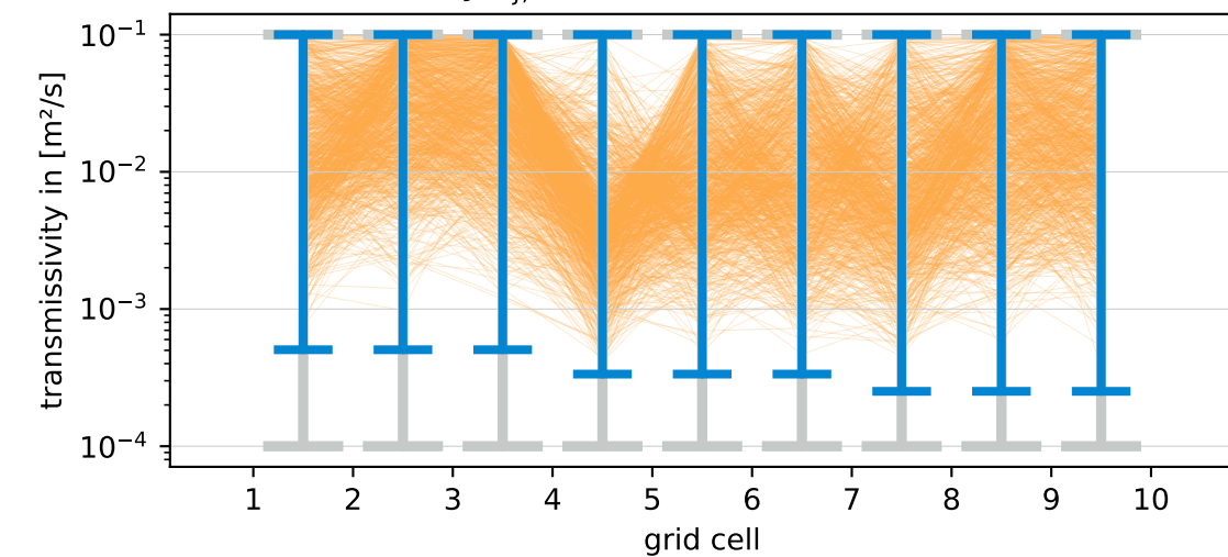
D : transmissivity T_{j,i}
