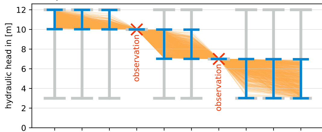
A : hydraulic heads h_i
